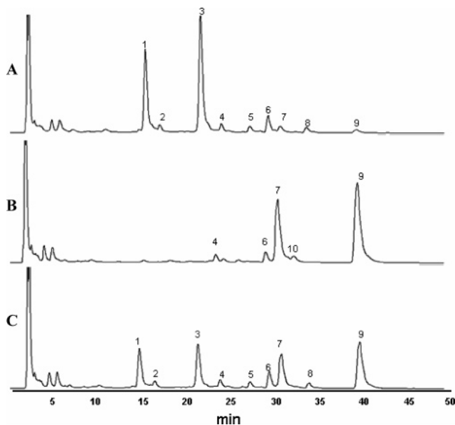
Figure 2. HPLC separation of isoflavonoids in crude soybean flour methanol extract: (A) crude soybean flour methanol extract (peaks: 1, daidzin; 2, glycitin; 3, genistin; 4, malonyldaidzin;* 5, acetyldaidzin;* 6, malonylgenistin; 7, daidzein; 8, acetylgenistin;* 9, genistein; 10, glycitein); (B, C) crude soybean flour methanol extract after 10 min of hydrolysis reaction with 0.001 unit of D. nigrescens \beta -glucosidase (B) or D. cochinchinensis \beta -glucosidase (C) in 0.1 M sodium acetate, pH 5.5. The digested and undigested methanol extracts were separated on analytical C 18 reverse phase HPLC as described under Materials and Methods. * These peaks were provisionally identified on the basis of their relative elution times in comparison to a previous study that used a similar solvent system and HPLC column (20).
